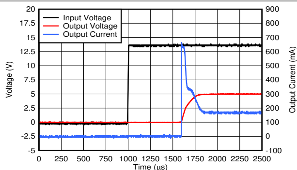
图 6-31. Startup Plot Inrush Current
