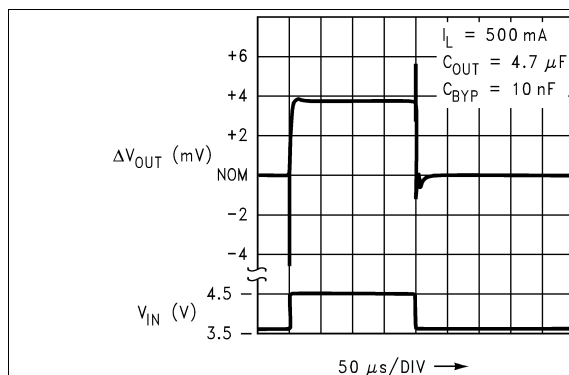
Figure 42. Line Transient Response
