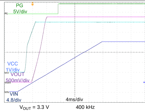
图 31. Start-Up Waveform
