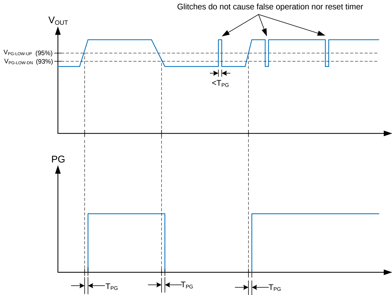
图 8. Static Power-Good Operation
