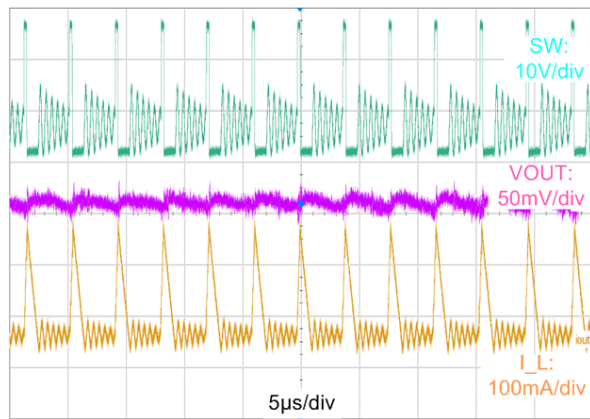
图 13. Typical PFM Switching Waveforms V_{IN} = 24\text{ V} , V_{OUT} = 5\text{ V} , I_{OUT} = 30\text{ mA}
