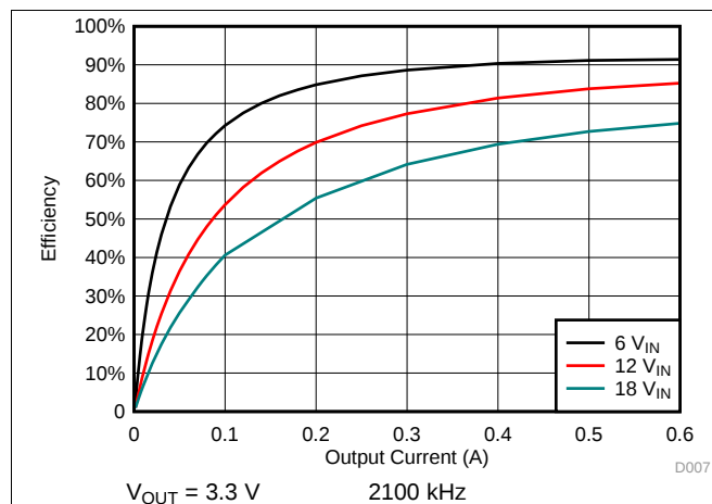
图 34. Efficiency
