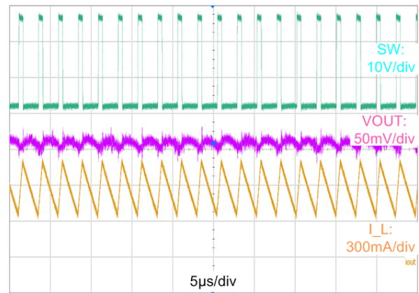
图 14. Typical PWM Switching Waveforms V_{IN} = 24\text{ V} , V_{OUT} = 5\text{ V} , I_{OUT} = 600\text{ mA} , f_S = 400\text{ kHz}
