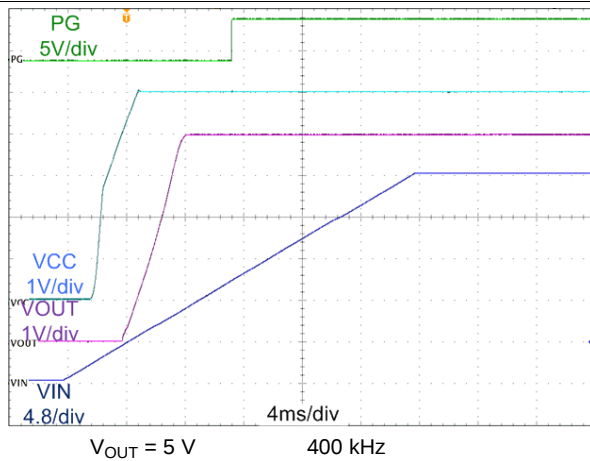
图 30. Start-Up Waveform
