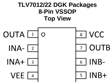
Pin Functions: TLV7012/22
