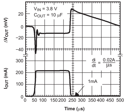
Figure 21. TPS73028 Load Transient Response
