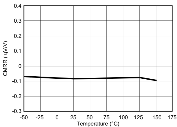
图 7-4. Common-Mode Rejection Ratio vs Temperature
