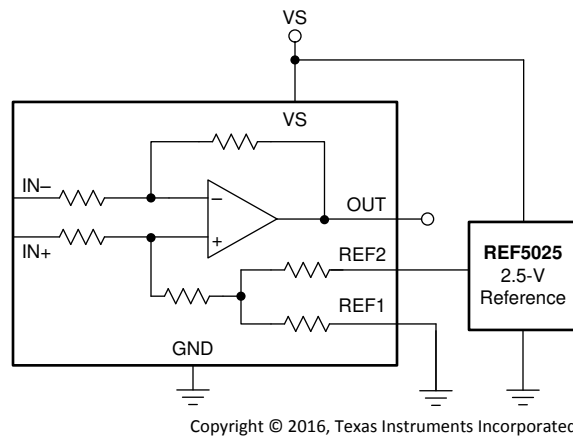
图 8-7. Mid-External Reference Output
