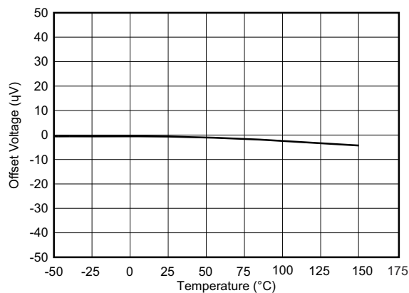
图 7-2. Offset Voltage vs Temperature
