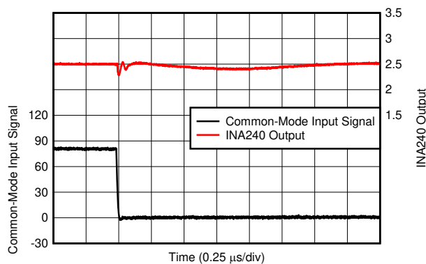
图 7-20. Step Response
