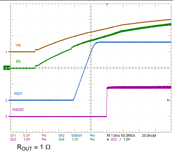
图 48. V IN Start-up
