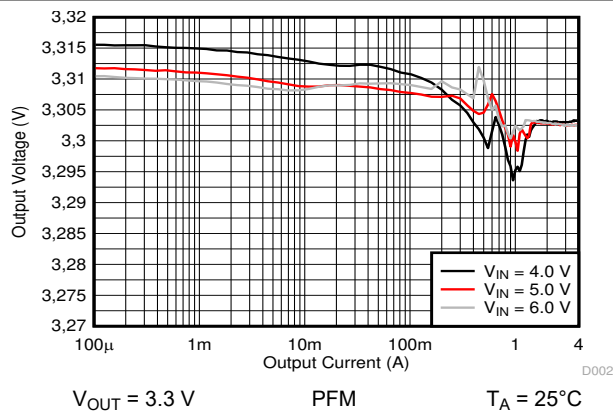
图 10-12. Output Voltage versus Output Current
