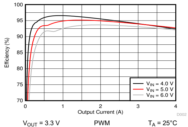
图 10-3. Efficiency versus Output Current
