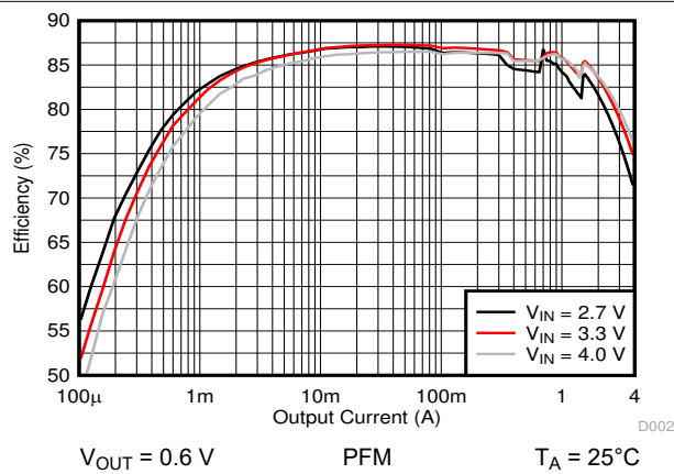
图 10-10. Efficiency versus Output Current
