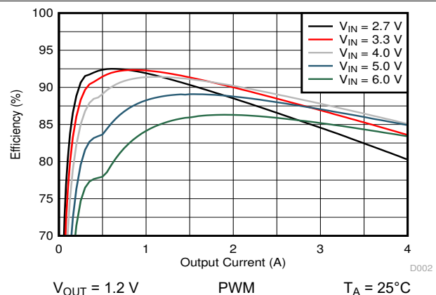
图 10-7. Efficiency versus Output Current
