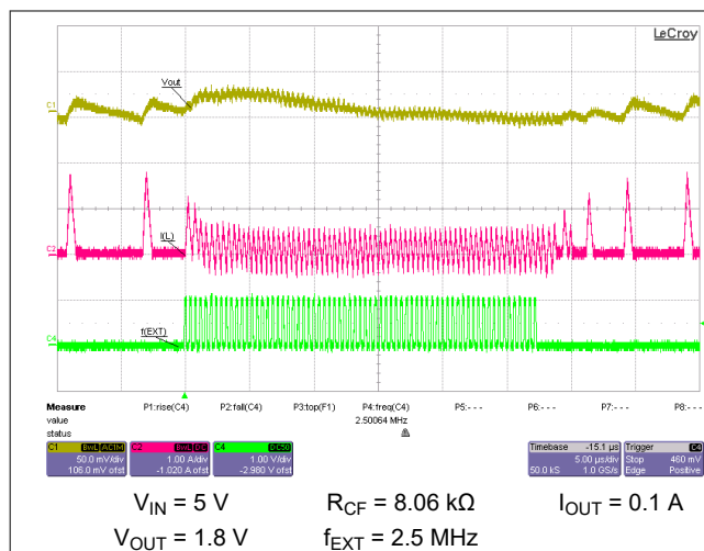
图 10-61. Switching from External Synchronization to Power-Save Mode (PFM)
