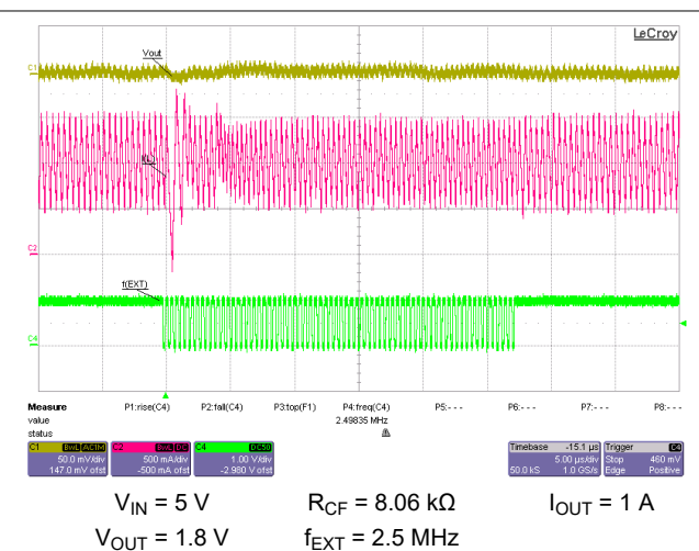
图 10-62. Switching from External Synchronization to Internal Fixed Frequency
