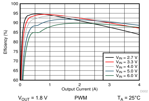
图 10-5. Efficiency versus Output Current
