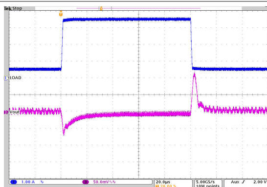
图 10-26. Load Transient Response
