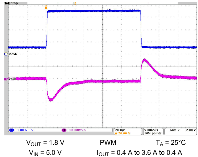
图 10-25. Load Transient Response
