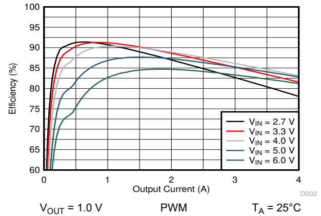
图 10-9. Efficiency versus Output Current
