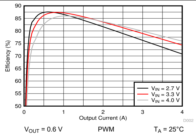
图 10-11. Efficiency versus Output Current
