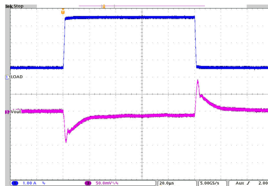
图 10-27. Load Transient Response
