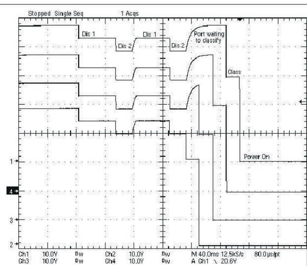
图 6-2. Four Port Discovery, Class, Power On
