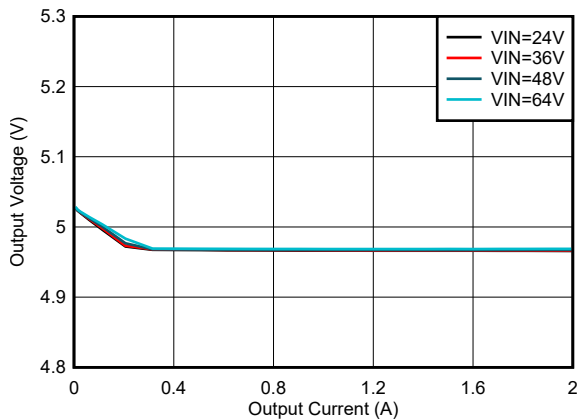
LMR38020 V_{OUT} = 5\text{ V} 400 kHz PFM Version
