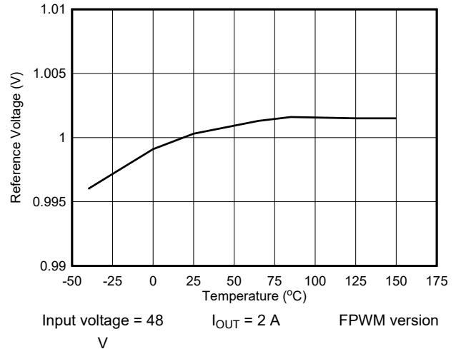
图 7-4. Reference Voltage vs Temperature
