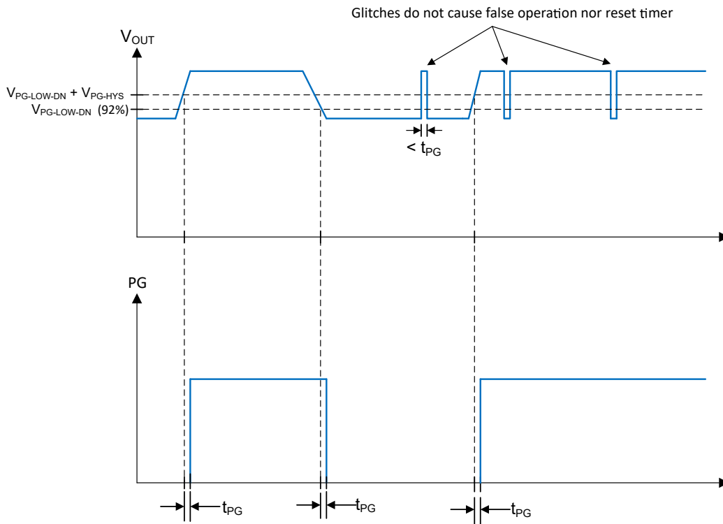
图 8-6. Power-Good-Timing Behavior
