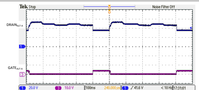
Figure 10-6. Semiauto Mode Discovery with a Valid Class 0-3 Load
