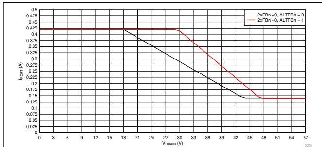
Figure 9-74. 1x Mode (2xFBn = 0) Foldback Curves, I PORT vs V DRAIN
