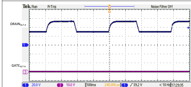
Figure 10-5. Open Circuit Detection Signature
