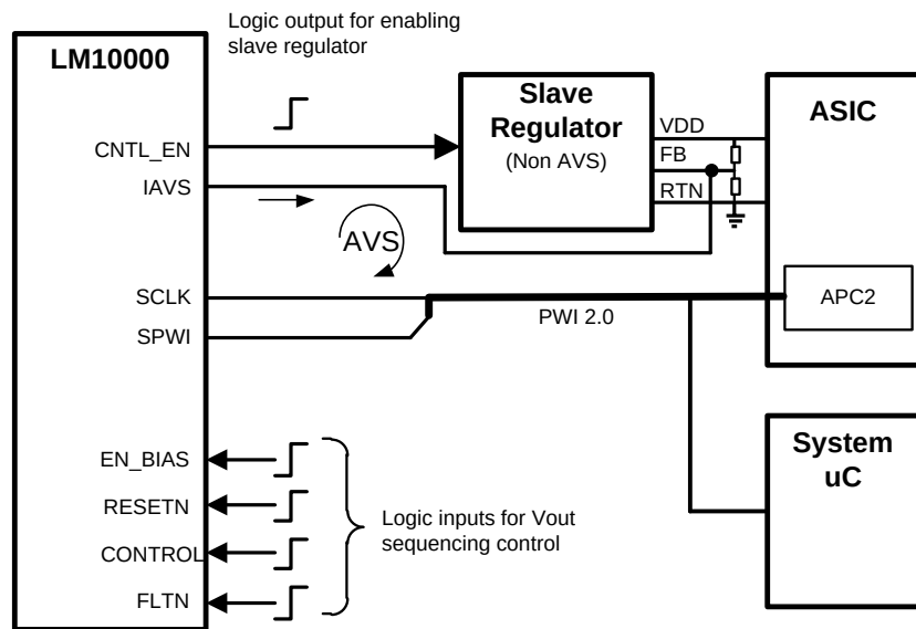
Figure 7. LM10000 provides flexible digital power management via multi-master PWT 2.0, and flexible V_{OUT} sequencing control
