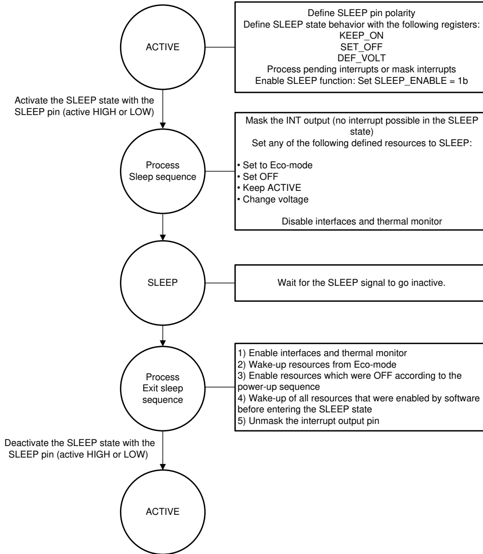
图 8-6. SLEEP Flow for CONFIG2 Pin Shorted LDOAO
