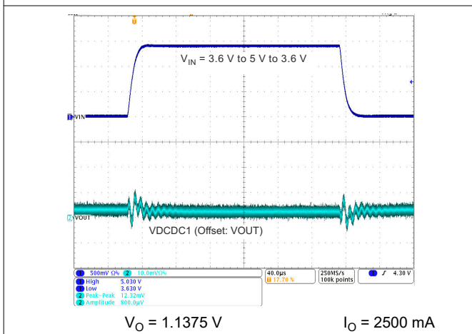
图 9-6. DCDC1 Line Transient Response
