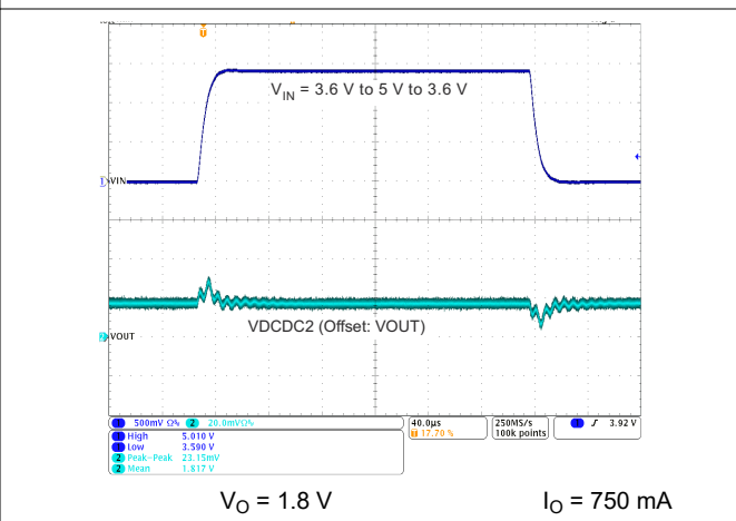
图 9-7. DCDC2 Line Transient Response
