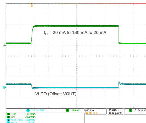
图 9-11. LDO1, LDO2, LDO3 Load Transient Response
