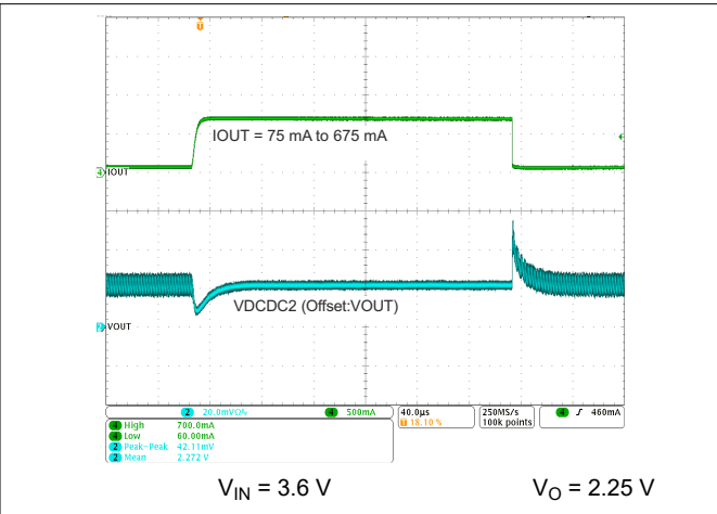
图 9-3. DCDC2 Load Transient Response
