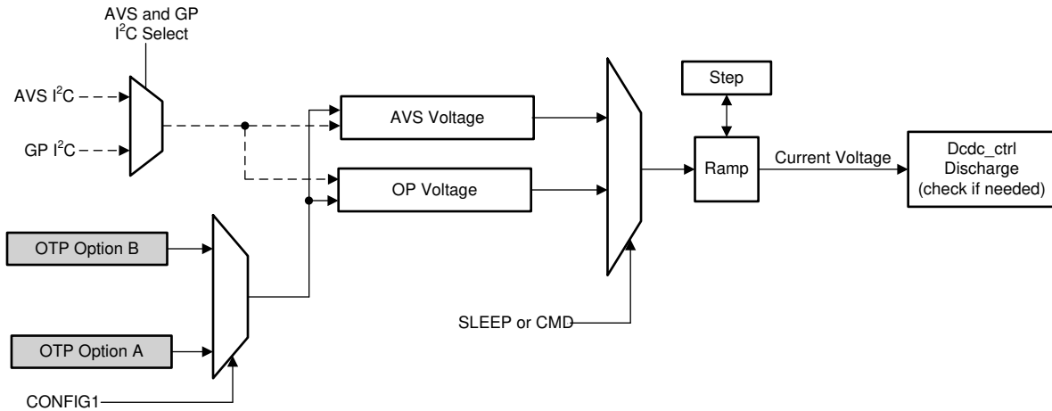
图 8-11. DC-DC Voltage Scaling Architecture
