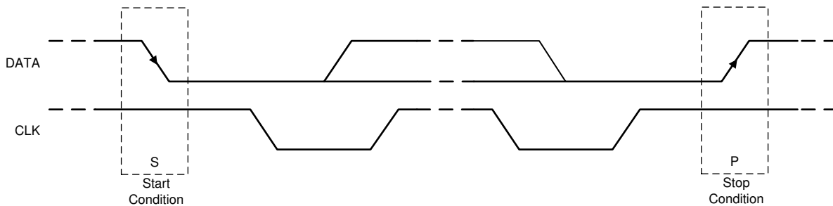
图 8-19. START and STOP Conditions
