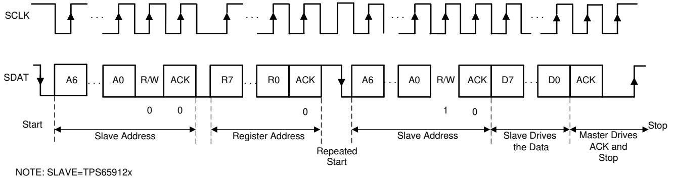
图 8-24. I 2 C Interface READ from TPS659128x; F/S Mode
