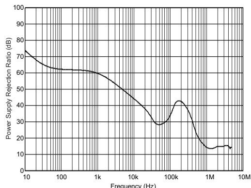
V_{IN} = 3.2\text{ V} V_{OUT} = 2.7\text{ V} I_{OUT} = 225\text{ mA}
