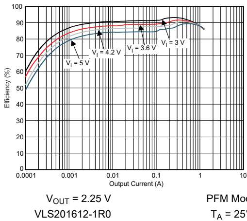
图 6-9. DCDC2 Efficiency vs Output Current
