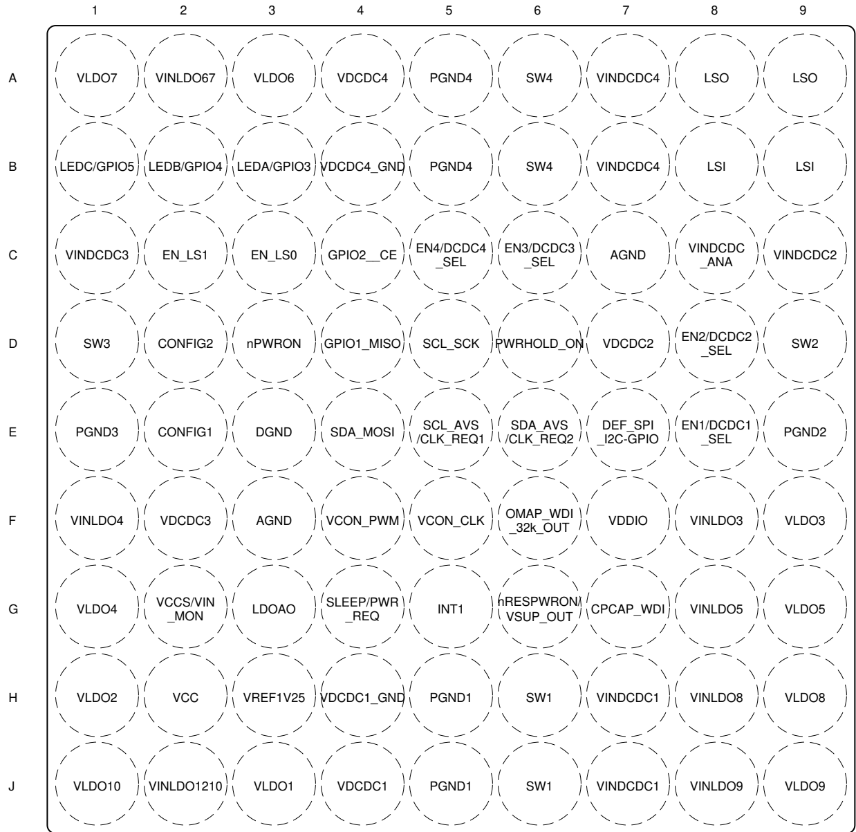
图 5-1. 81-Pin YFF DSBGA (Bottom View)
