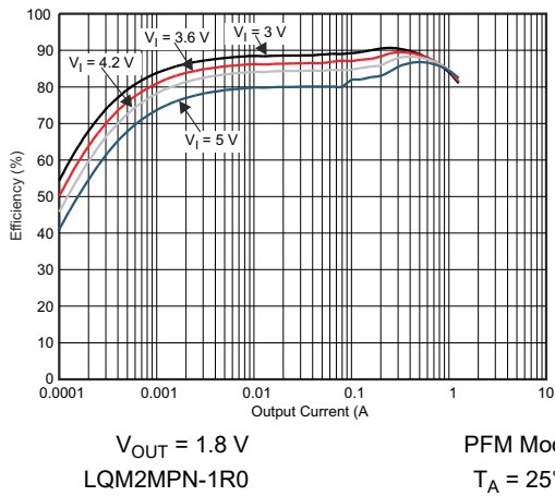
图 6-7. DCDC2 Efficiency vs Output Current
