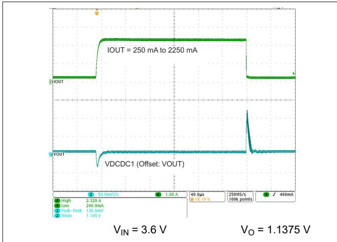
图 9-2. DCDC1 Load Transient Response
