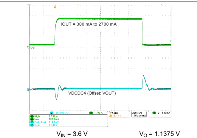
图 9-5. DCDC4 Load Transient Response
