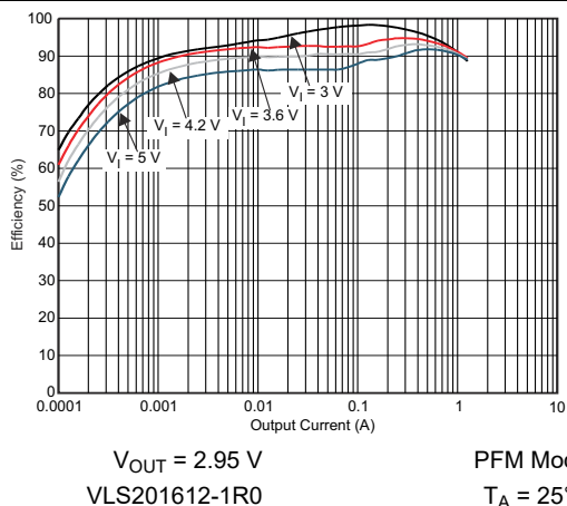
图 6-11. DCDC2 Efficiency vs Output Current
