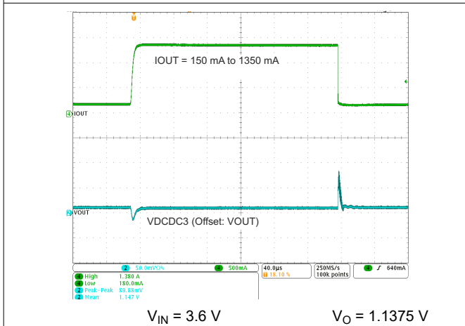
图 9-4. DCDC3 Load Transient Response
