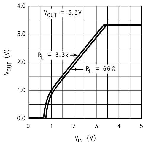
Figure 5. Dropout Characteristics
