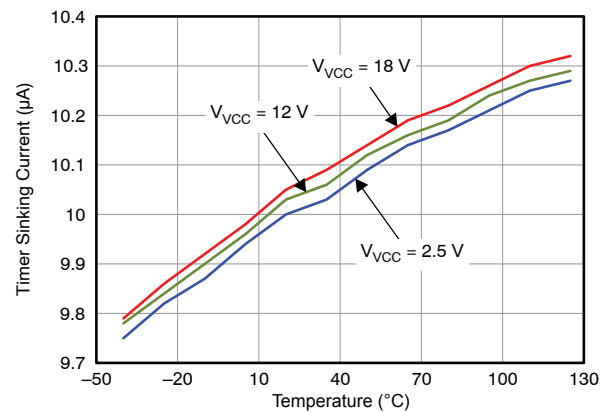
Figure 22. Timer Sinking Current vs V_{CC} and Temperature
