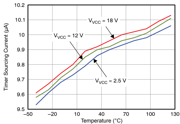
Figure 21. Timer Sourcing Current vs V_{CC} and Temperature
