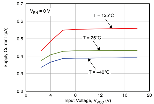
Figure 18. Supply Current vs V_{CC} and Temperature When V_{EN} Pulled Low
