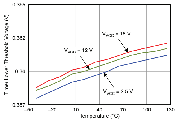
Figure 20. Timer Lower Threshold vs V_{CC} and Temperature
