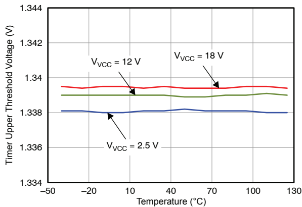
Figure 19. Timer Upper Threshold vs V_{CC} and Temperature
