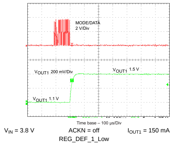
Figure 35. V OUT1 Change With EasyScale Interface
