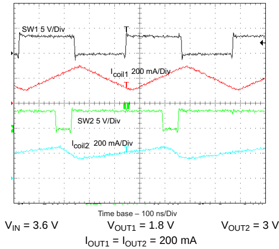
Figure 33. Typical Operation
