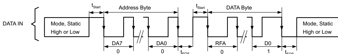
Figure 10. EasyScale Protocol Without Acknowledge
