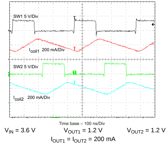
Figure 34. Typical Operation
