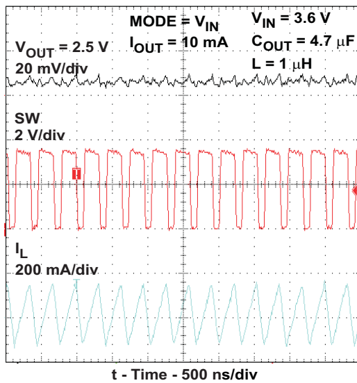
Figure 37. Forced PWM Mode Operation I_{OUT} = 10\text{mA}
