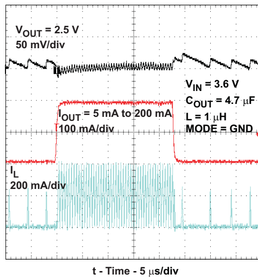
Figure 44. Load Transient Response 5mA to 200mA PFM to PWM Mode, V_{OUT} 2.5V
