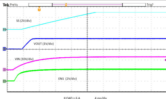
图 8-41. Power Up with V_{IN}
