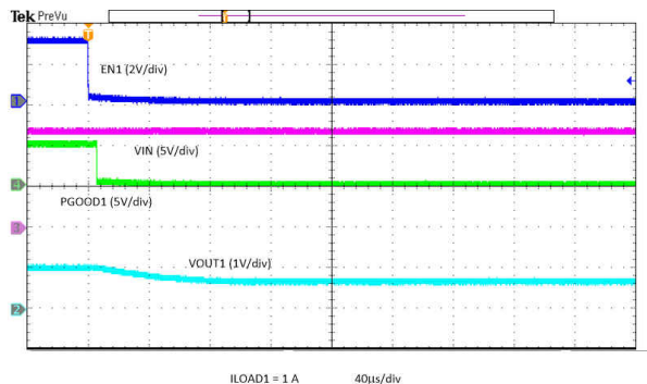
图 8-21. Power Down with EN 1 with Pre Bias
