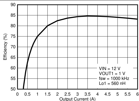
图 8-3. V OUT1 Efficiency
