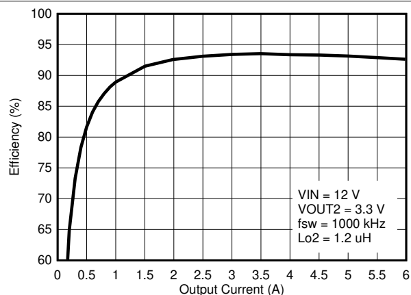
图 8-4. V OUT2 Efficiency
