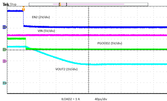
图 8-22. Power Down with EN 2 with Pre Bias
