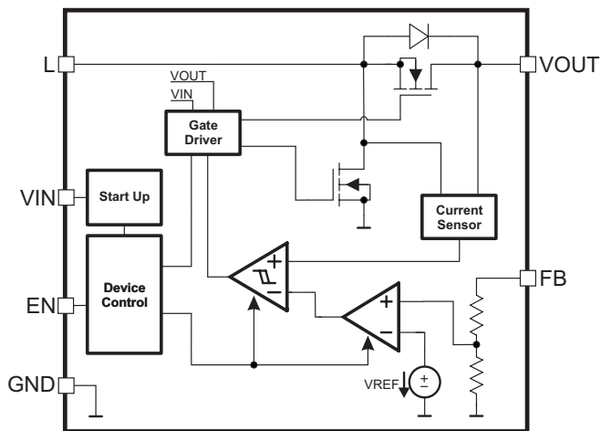
Figure 24. Functional Block Diagram (Fixed Output Voltage Version)
