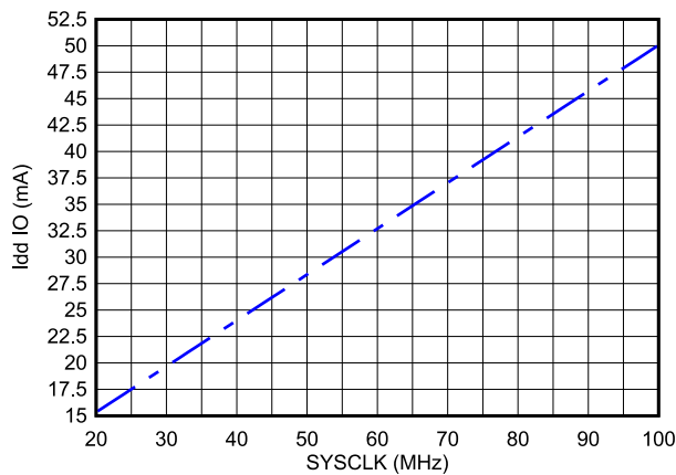
图 7-2. Operating Current Versus Frequency
