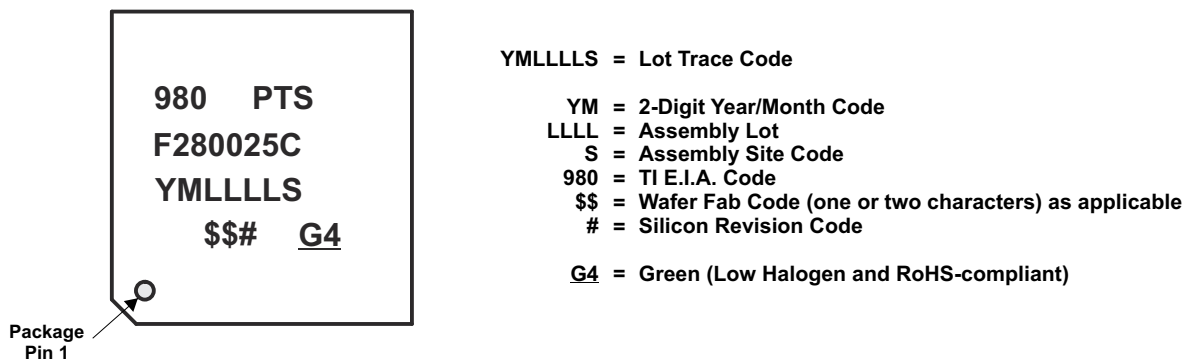
图 10-3. Package Symbolization for PT Package
