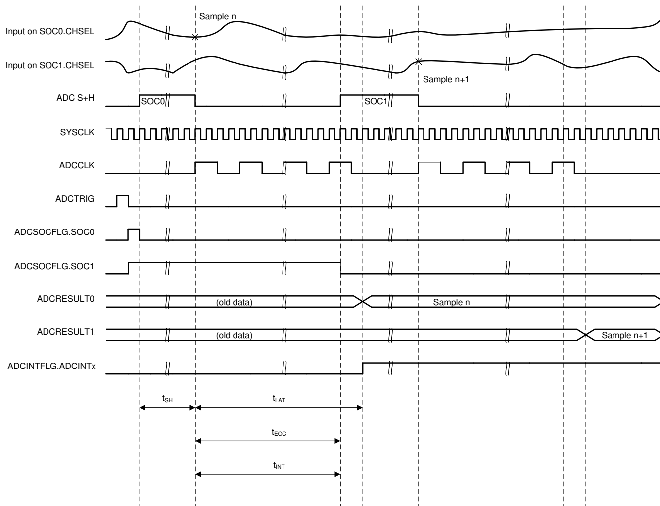
图 7-35. ADC Timings
