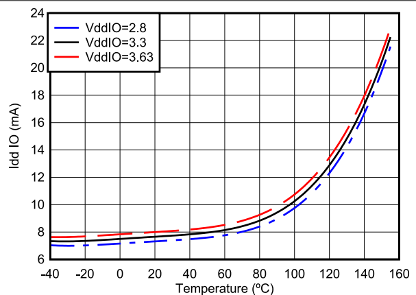
图 7-5. Current Versus Temperature - STANDBY Mode
