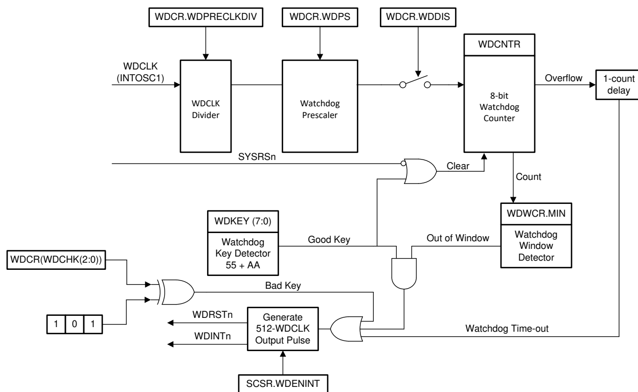
图 8-3. Windowed Watchdog
