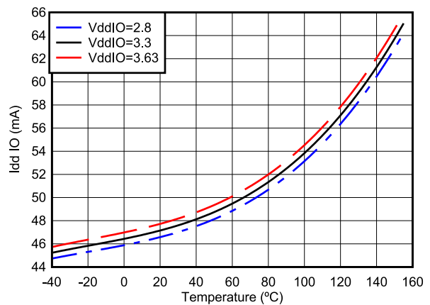
图 7-3. Operating Current Versus Temperature
