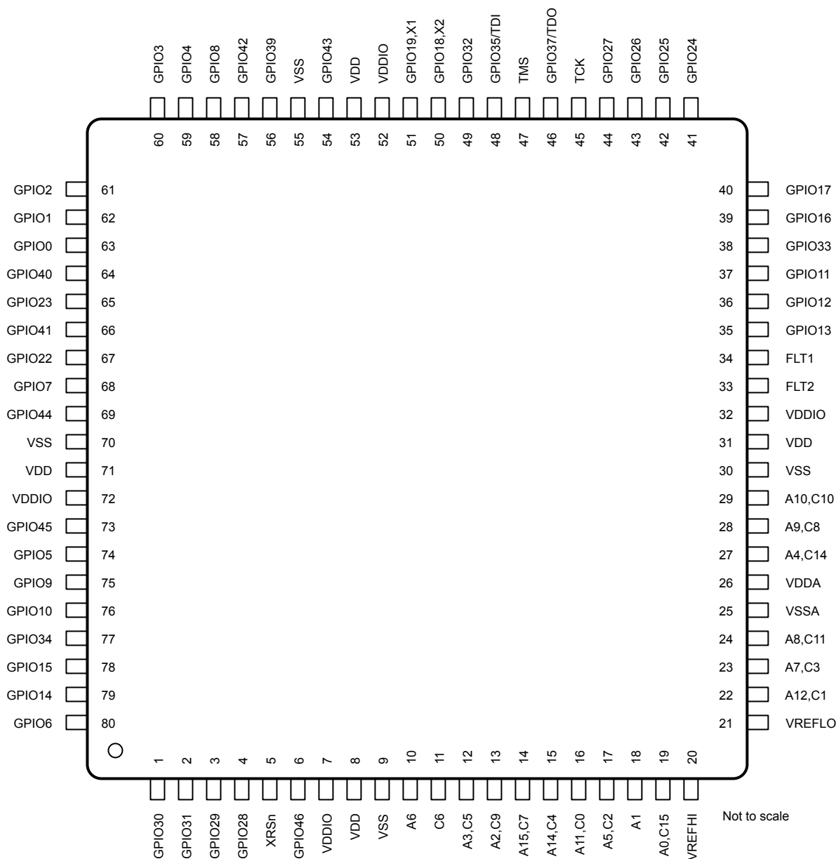
图 6-1. 80-Pin PN Low-Profile Quad Flatpack (Top View)
