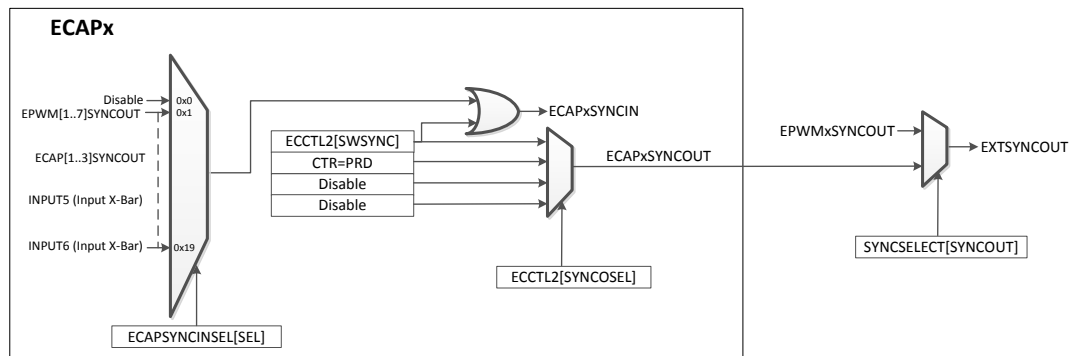
图 7-48. eCAPsynchronization Scheme
