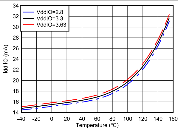
图 7-4. Current Versus Temperature - IDLE Mode
