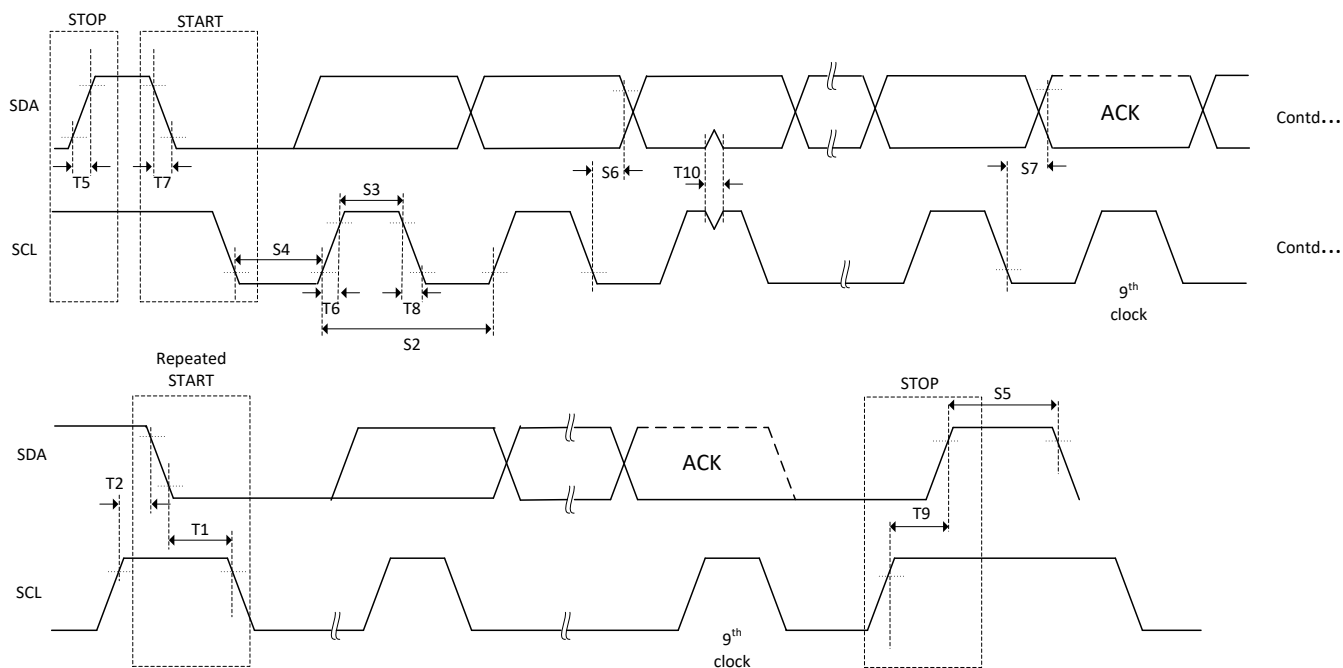
图 7-54. I2C Timing Diagram
