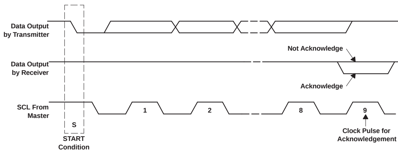
Figure 47. Acknowledge on the I²C Bus
