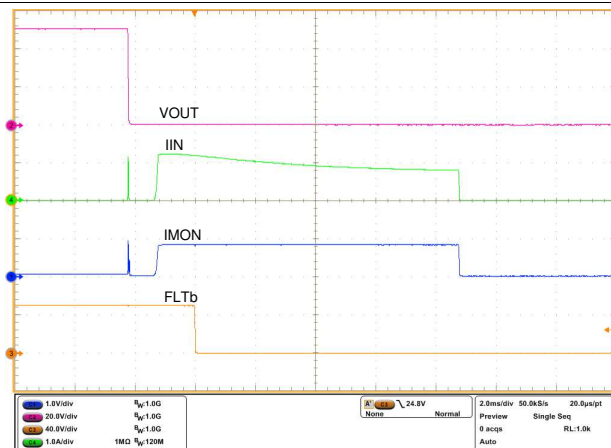
图 32. Overload Performance During Load Step from 140 \Omega to 40 \Omega
