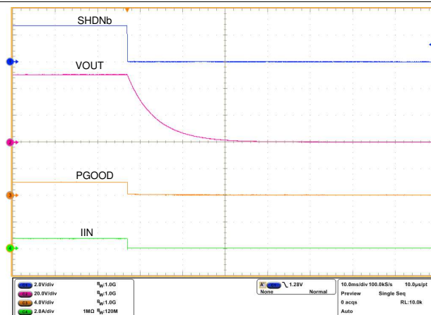
图 36. Turn OFF using \overline{\text{SHDN}} Control
