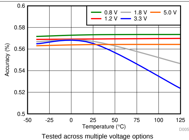
图 7. Undervoltage Hysteresis Voltage Accuracy vs Temperature
