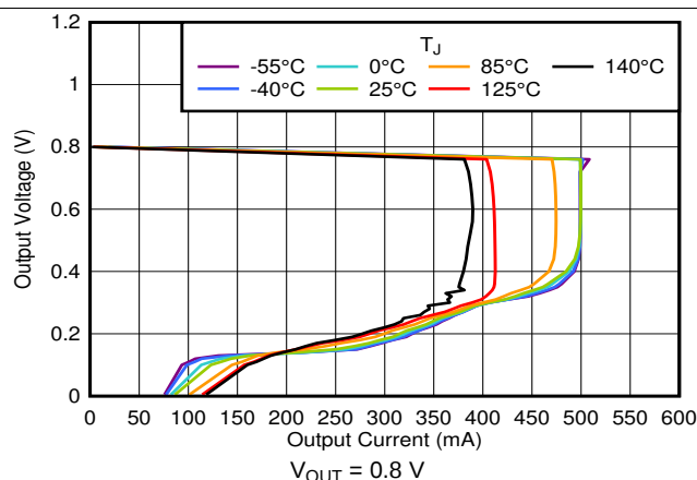
图 36. Foldback Current Limit vs I_{OUT} and Temperature
