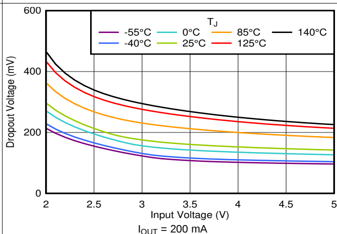
图 34. Dropout vs V_{IN} and Temperature
