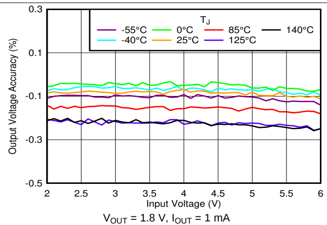
图 26. Output Accuracy vs V_{IN} and Temperature
