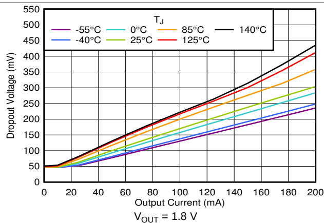
图 32. Dropout vs I_{OUT} and Temperature
