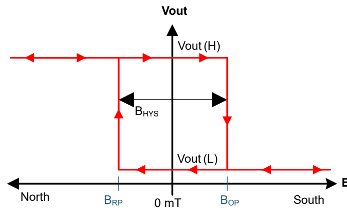
图 8-2. Latch Functionality
