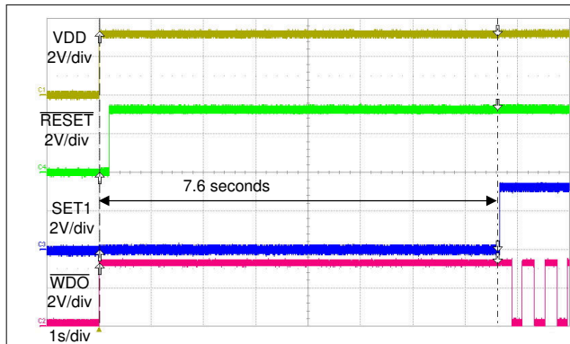
图 8-13. Startup Without a WDI Signal
