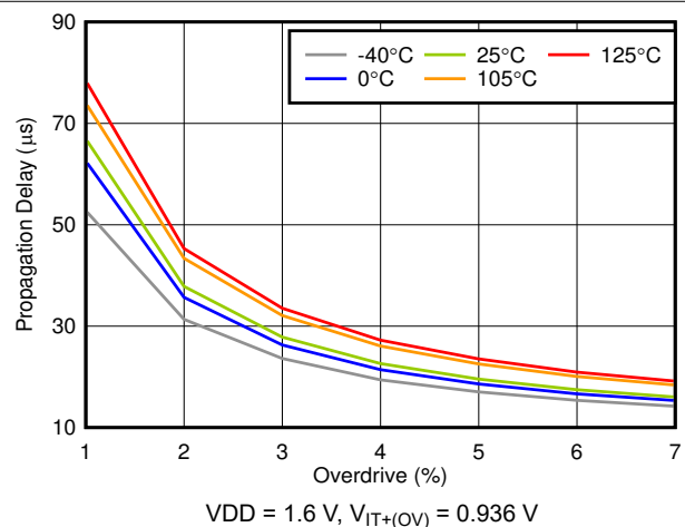
图 6-14. Propagation Delay vs Overdrive
