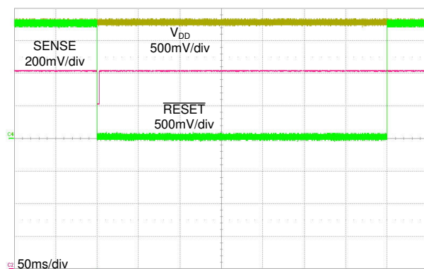
图 8-11. Typical \overline{\text{RESET}} Delay Timing
