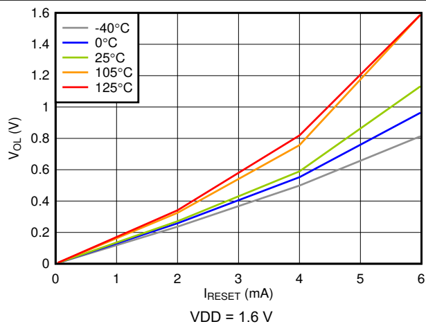
图 6-12. Low-Level RESET Voltage vs RESET Current
