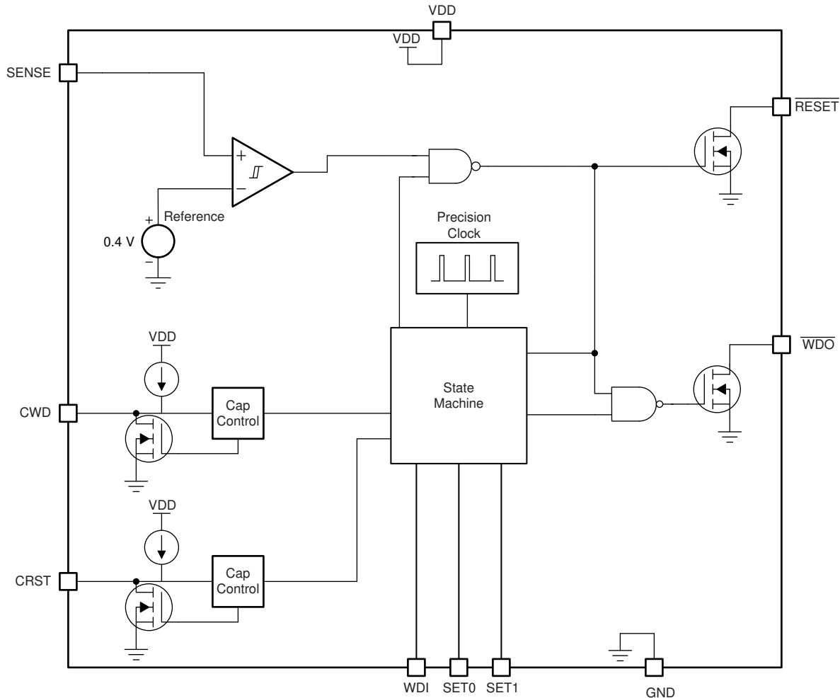
图 7-2. Adjustable Version Block Diagram
