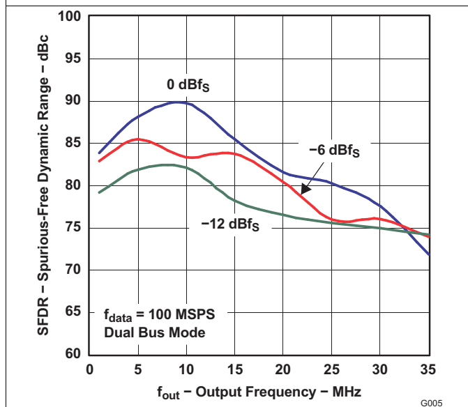
Figure 5. Spurious-Free Dynamic Range vs Output Frequency
