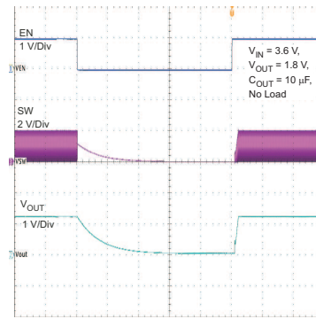
Time Base - 2ms/Div
