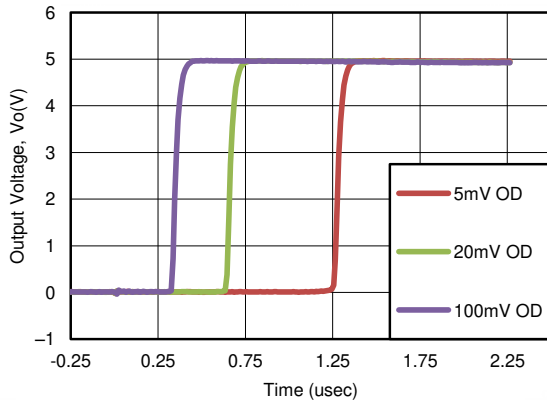
图 8-2. Response Time for Various Overdrives (Positive Transition)
