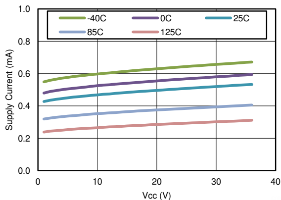
图 6-1. Supply Current vs Supply Voltage
