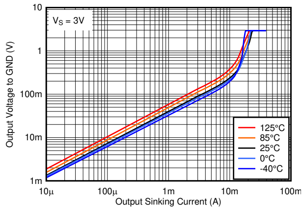
图 6-22. Output Low Voltage vs. Output Sinking Current at 3V
