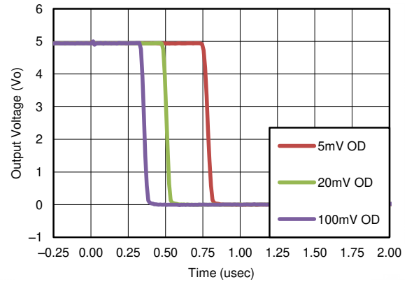
图 8-3. Response Time for Various Overdrives (Negative Transition)
