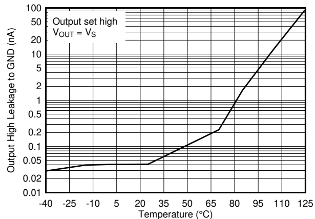
图 6-26. Output High Leakage Current vs. Temperature at 5V
