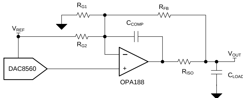
Figure 71. Bipolar Output Range Using Internal Reference
