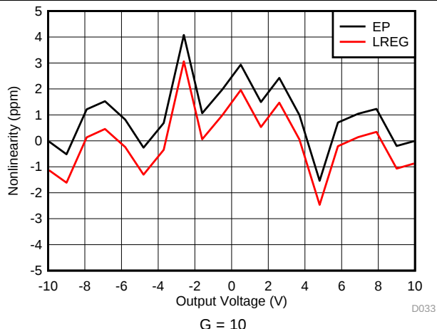
图 34. Gain Nonlinearity
