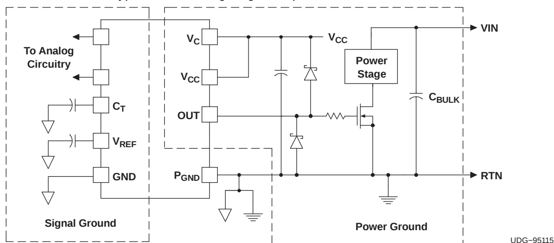
Figure 13. Ground Planes
