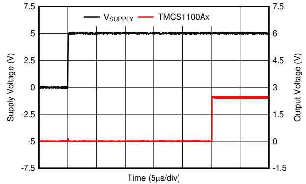
图 7-20. Startup Transient Response
