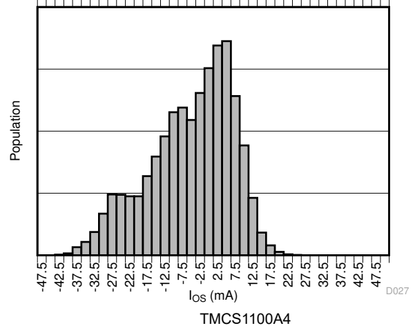
图 7-8. Input Offset Current Production Distribution
