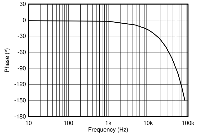
图 7-10. Phase vs. Frequency, All Gains
