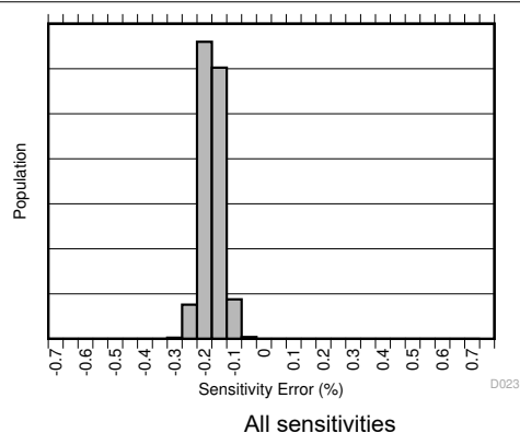
图 7-4. Sensitivity Error Production Distribution
