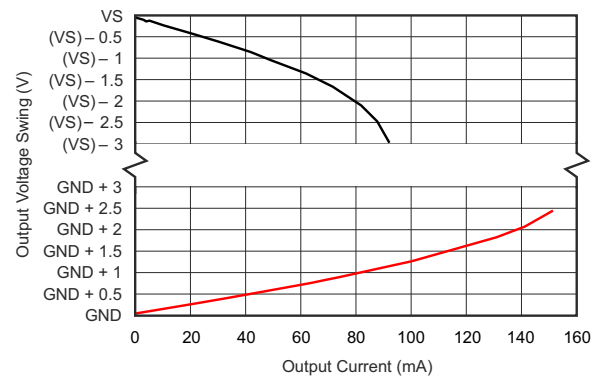
图 7-12. Output Swing vs. Output Current
