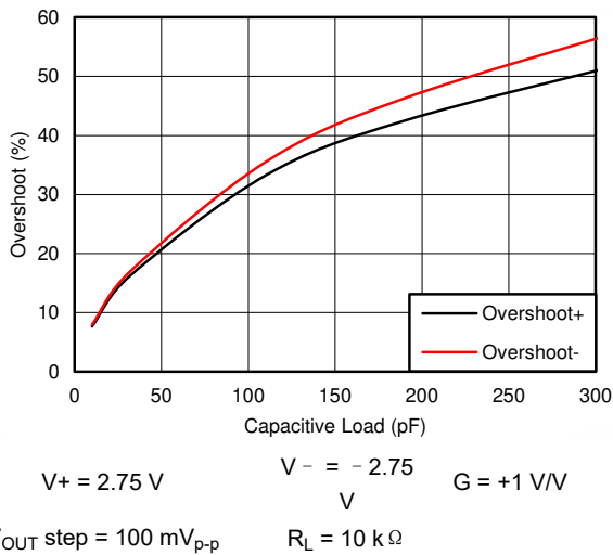
图 8-23. Small-Signal Overshoot vs Load Capacitance
