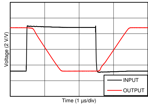
图 8-26. Overload Recovery
