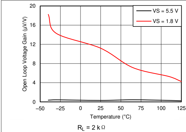
图 8-7. Open-Loop Gain vs Temperature
