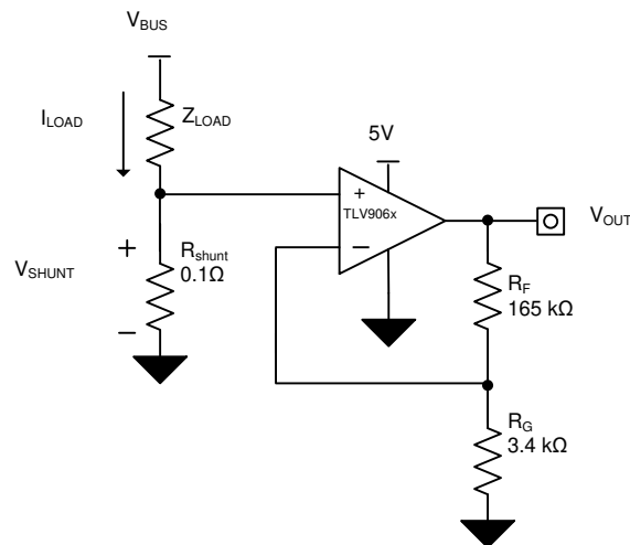
图 10-1. TLV906x-Q1 in a Low-Side, Current-Sensing Application
