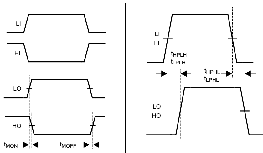
Figure 1. Timing Diagram
