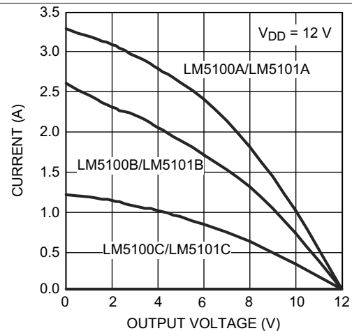
Figure 5. Source Current vs Output Voltage
