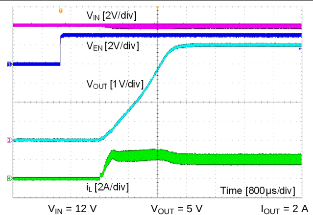
Figure 29. Start-Up by V_{EN}
