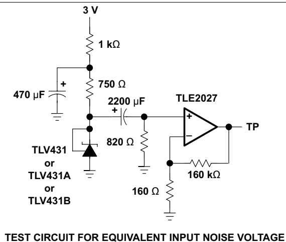
TEST CIRCUIT FOR EQUIVALENT INPUT NOISE VOLTAGE
