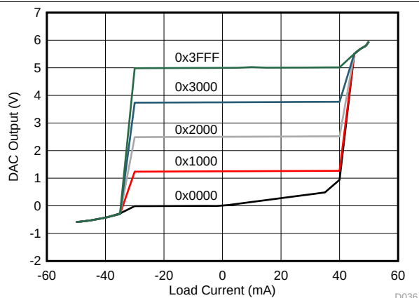
Figure 34. Source and Sink Capability with Gain = 1/2
