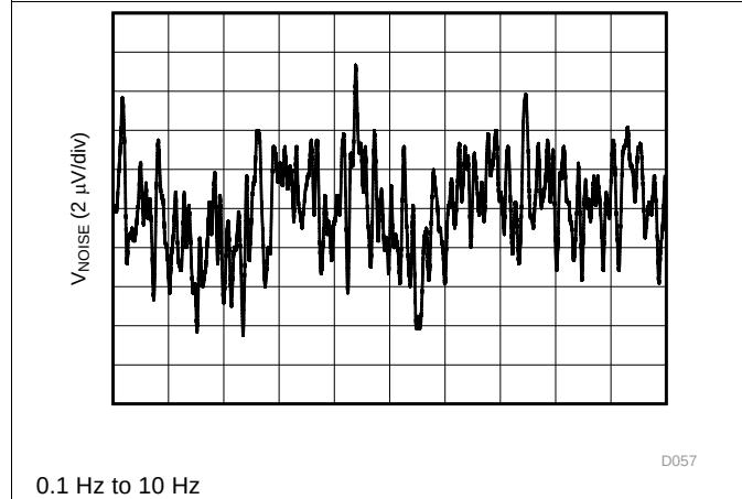
Figure 57. Internal Reference Noise
