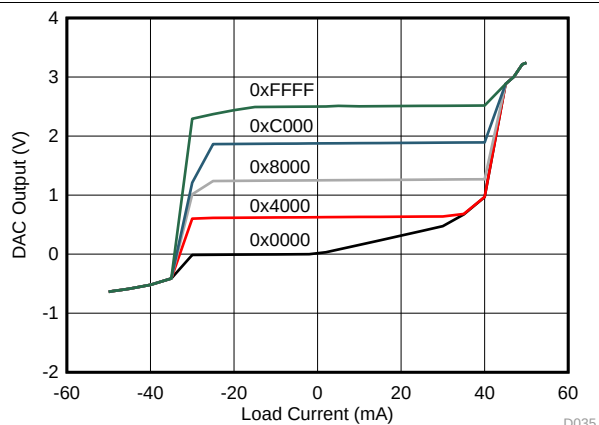
Figure 33. Headroom/Footroom vs Load Current
