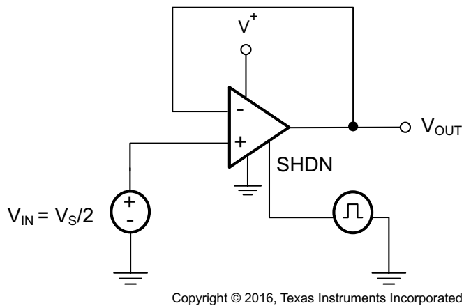
Figure 44. Turnon Time
