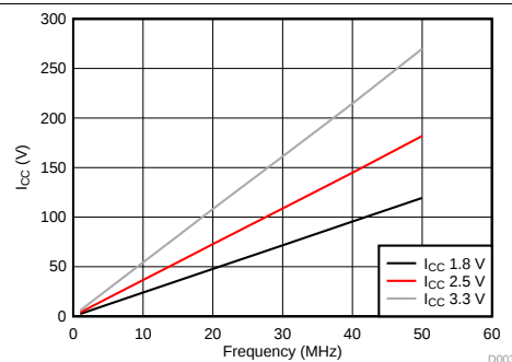
Figure 6. I CC vs Frequency
