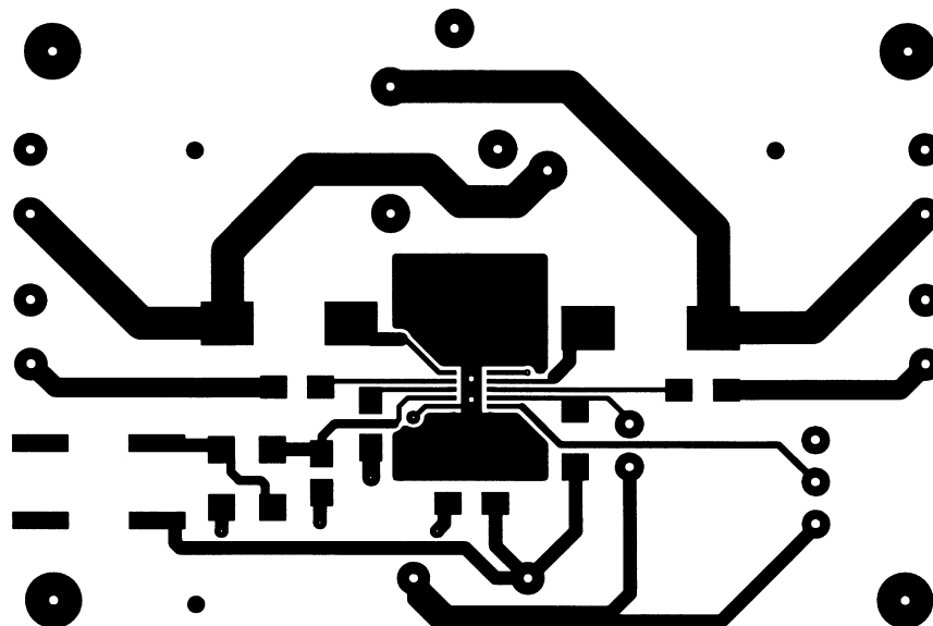
Figure 47. Recommended WSON/SO8 PC Board Layout: TOP Top Layer
