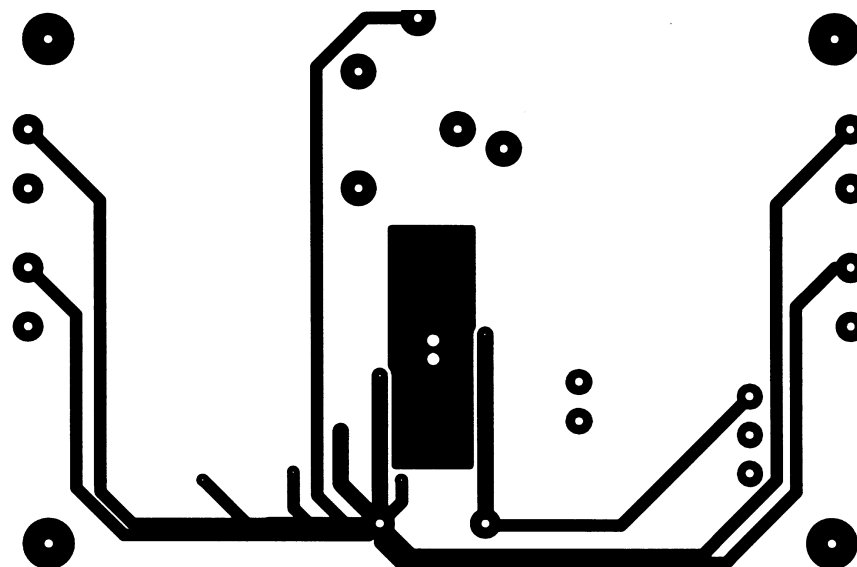
Figure 48. Recommended WSON/SO8 PC Board Layout: Bottom Layer
