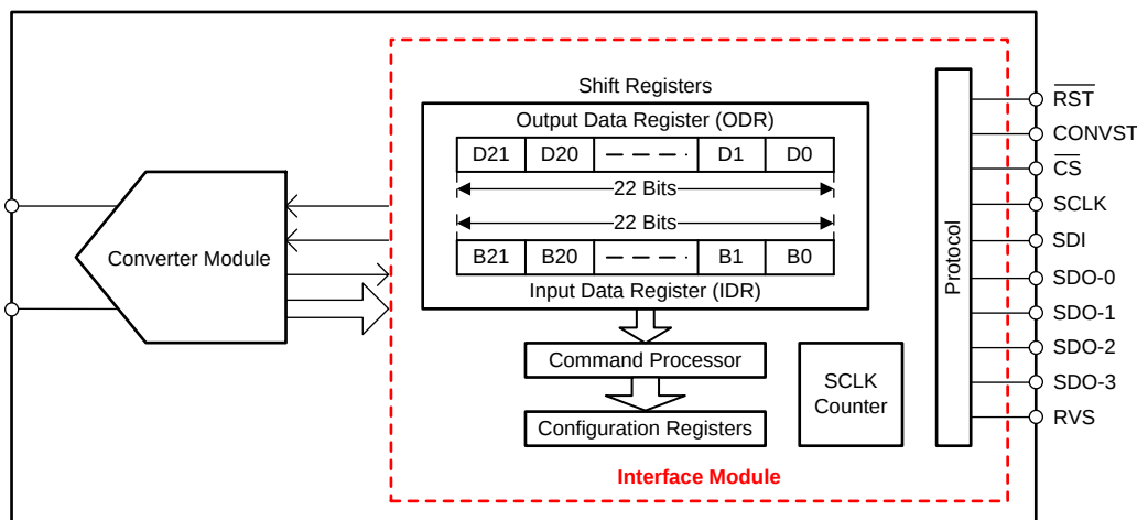
Figure 39. Interface Module
