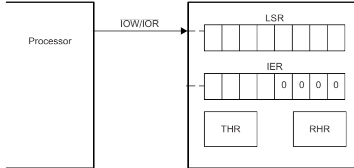
Figure 21. FIFO Polled Mode Operation
