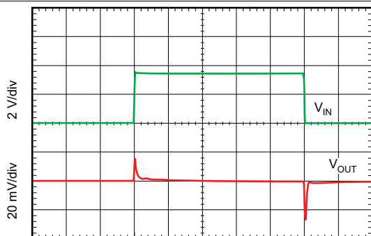
图 33. Line Transient Response
