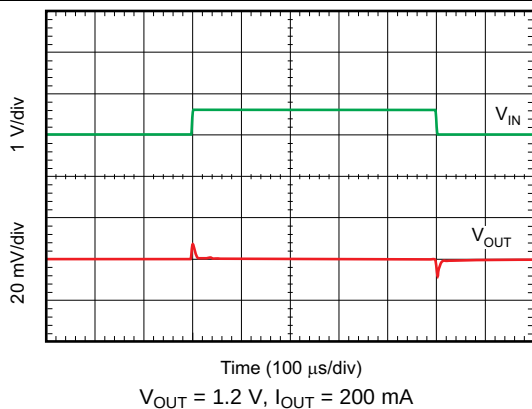
图 49. Line Transient Response
