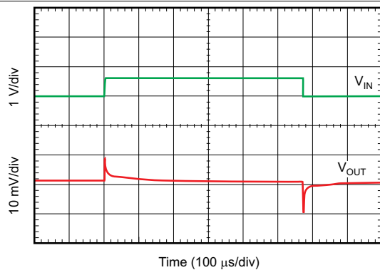
图 37. Line Transient Response
