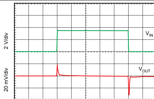
图 34. Line Transient Response
