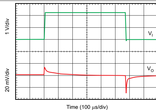
图 38. Line Transient Response
