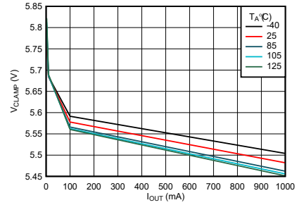
图 7-27. OVC Clamping Voltage (OVCSEL = Open) vs Load Current
