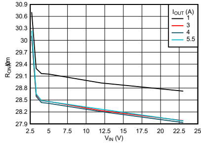
图 7-2. ON-Resistance vs Supply Voltage
