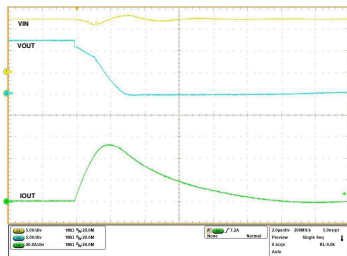
V_{IN} = 12\text{ V} , R_{ILM} = 549\text{ }\Omega , V_{EN/UVLO} = 3.3\text{ V} , I_{OUT} stepped from Open \rightarrow Short-circuit to GND
