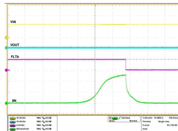
V_{IN} = 12\text{ V} , C_{OUT} = \text{Open} , I_{OUT} short-circuit to GND, R_{ILM} = 1650\text{ }\Omega , V_{EN/UVLO} stepped from 0\text{ V} to 3.3\text{ V}
