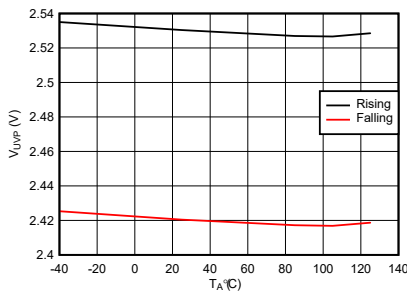
图 7-8. IN Undervoltage Threshold vs Temperature
