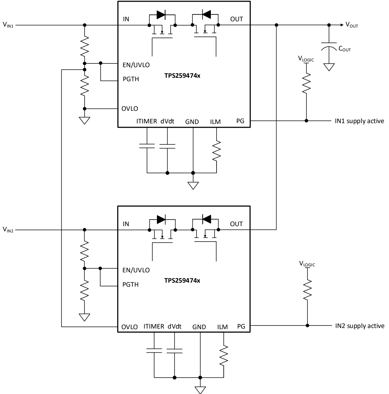
图 9-15. Priority power MUXing with 2 x TPS25947x
