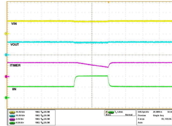
V_{IN} = 12\text{ V} , C_{ITIMER} = 2.2\text{ nF} , C_{OUT} = 470\text{ }\mu\text{F} , R_{ILM} = 549\text{ }\Omega , I_{OUT} ramped from 4\text{ A} \rightarrow 8\text{ A} \rightarrow 4\text{ A} within 1\text{ ms}
