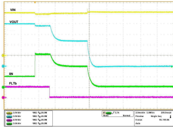
V_{IN} = 12\text{ V} , C_{ITIMER} = 2.2\text{ nF} , C_{OUT} = 220\text{ }\mu\text{F} , R_{ILM} = 549\text{ }\Omega , I_{OUT} stepped from 3\text{ A} \rightarrow 9\text{ A}
