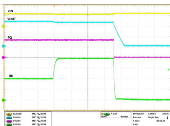
V_{IN} = 12\text{ V} , C_{ITIMER} = 2.2\text{ nF} , C_{OUT} = 470\text{ }\mu\text{F} , R_{ILM} = 549\text{ }\Omega , I_{OUT} ramped from 4\text{ A} \rightarrow 8\text{ A}
