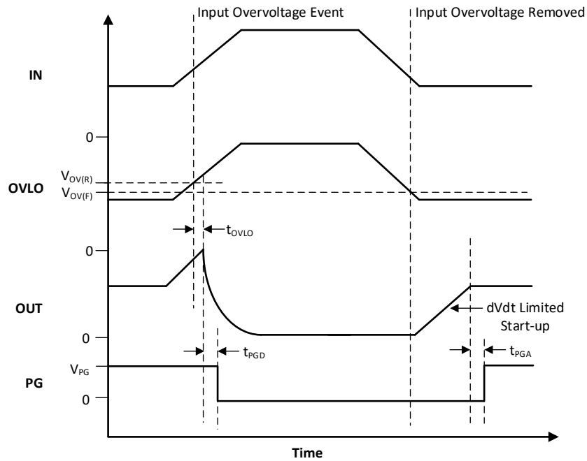
图 8-7. TPS259474x Overvoltage Lockout and Recovery
