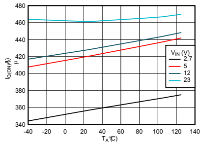
图 7-4. IN Quiescent Current vs Temperature (TPS259470x/4x Variants)
