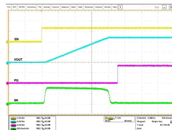
图 7-39. Start Up with Supply
