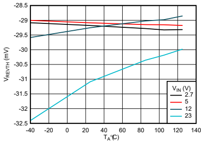
图 7-20. RCB - Reverse Comparator Threshold vs Temperature
