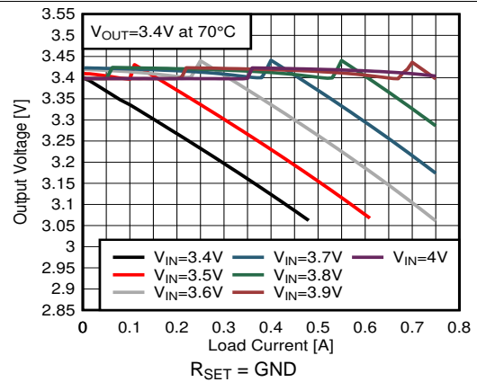
图 31. Output Voltage versus Load Current V OUT = 3.4 V
