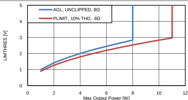
Figure 21. Max Output Power vs LIMTHRES, 8 Ω, PVCC = 13 V
