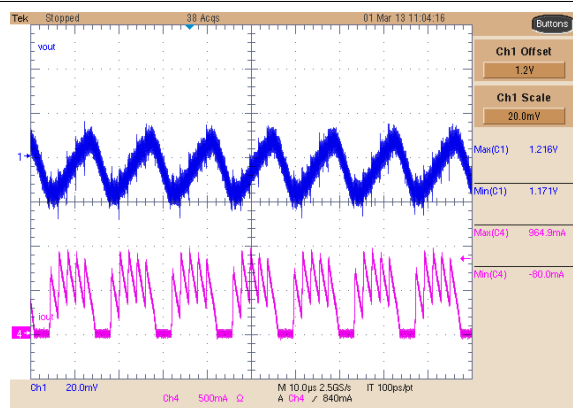
图 8-20. Buck 1 Low-Power Operation
