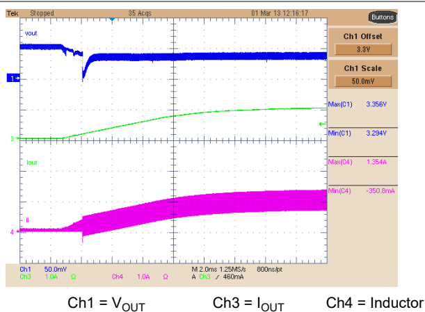
图 8-49. Buck 3 PWM to PFM Transition
