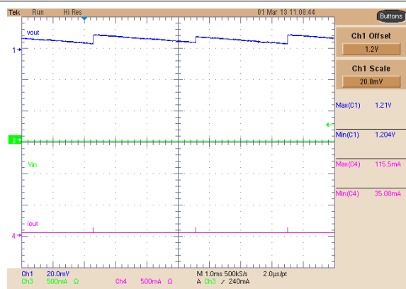
图 8-19. Buck 1 Low-Power Output, No Load
