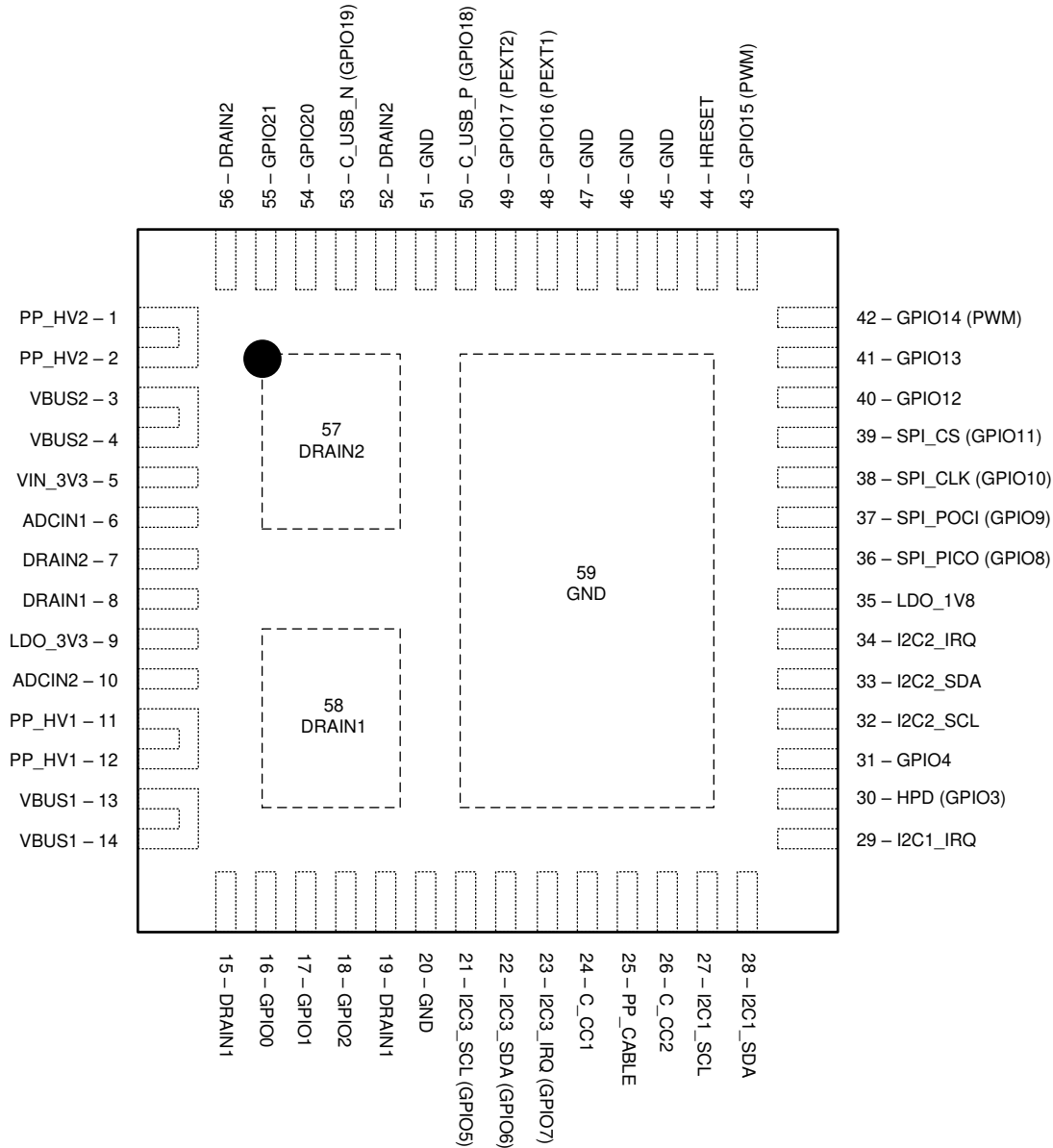
图 5-1. RSH Package 56-Pin QFN Top View
